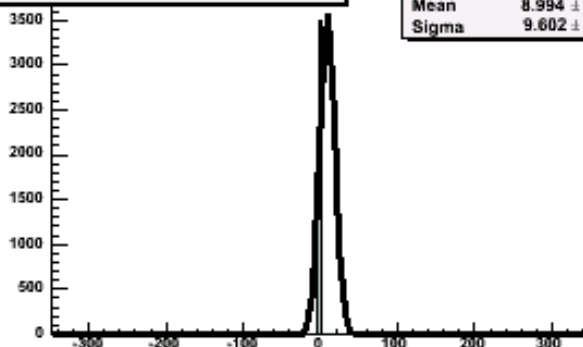
Difference between Original function and Minuit fit
