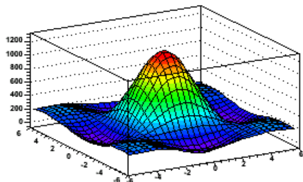
Minuit fit result on the Graph2D points
