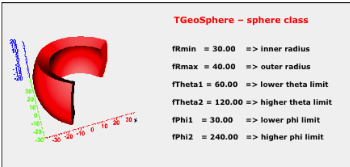
Figure 18.18: TGeoSphere Class
