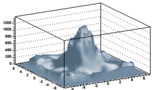
Histogram produced with Delaunay interpolation
