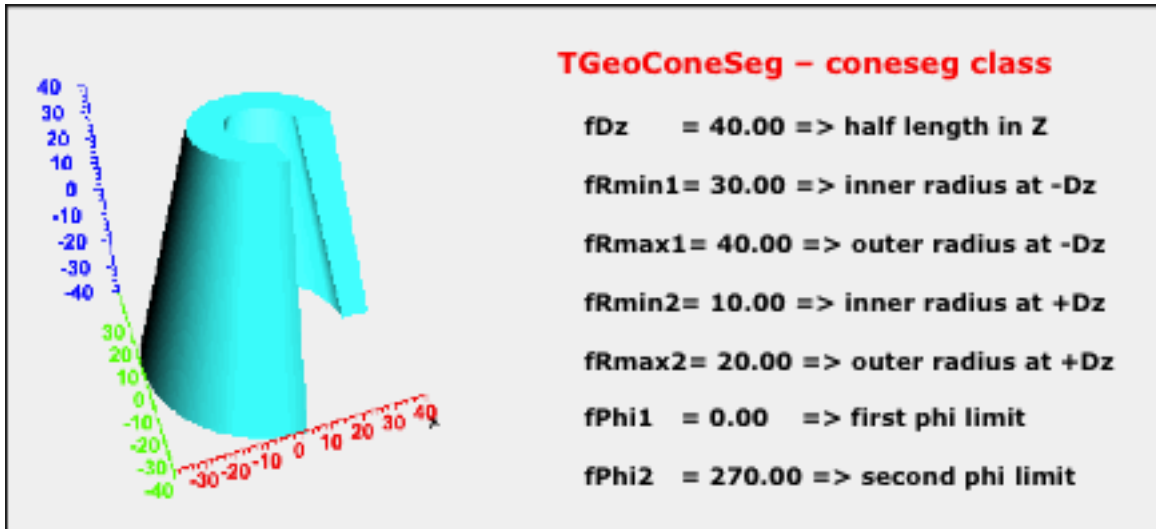
Figure 18.17: TGeoConeSeg Class
