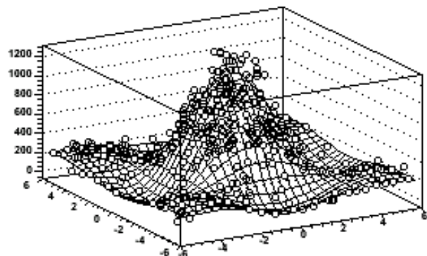
Original function with Graph2D points on top
