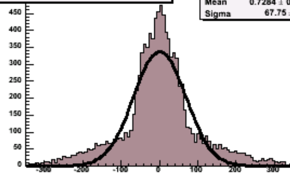
Difference between Original function and Function with noise
