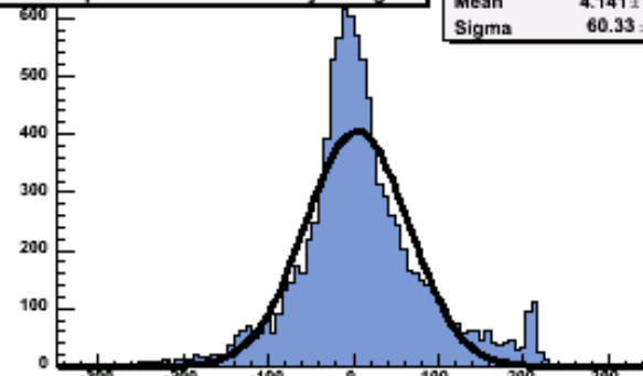
Difference between Original function and Interpolation with Delaunay triangles
