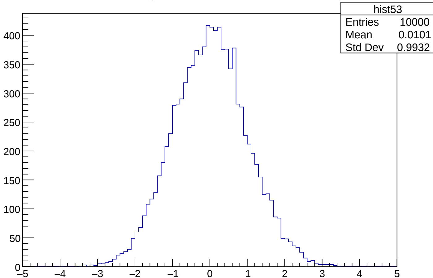
Histogram with random data
