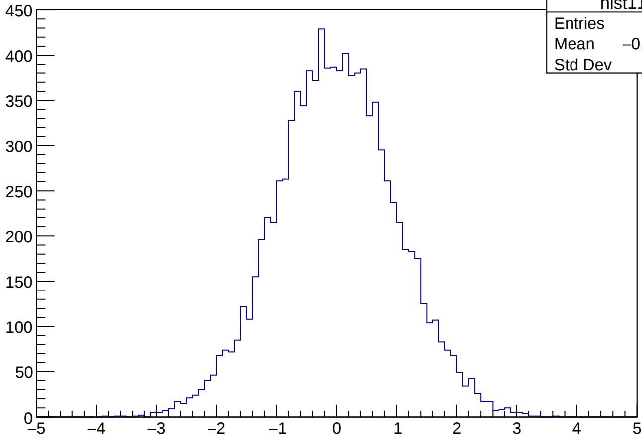
Histogram with random data
