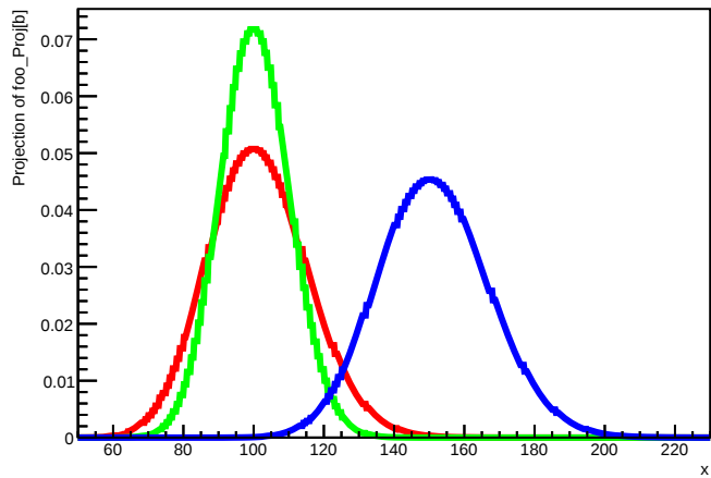
A RooPlot of "x"
