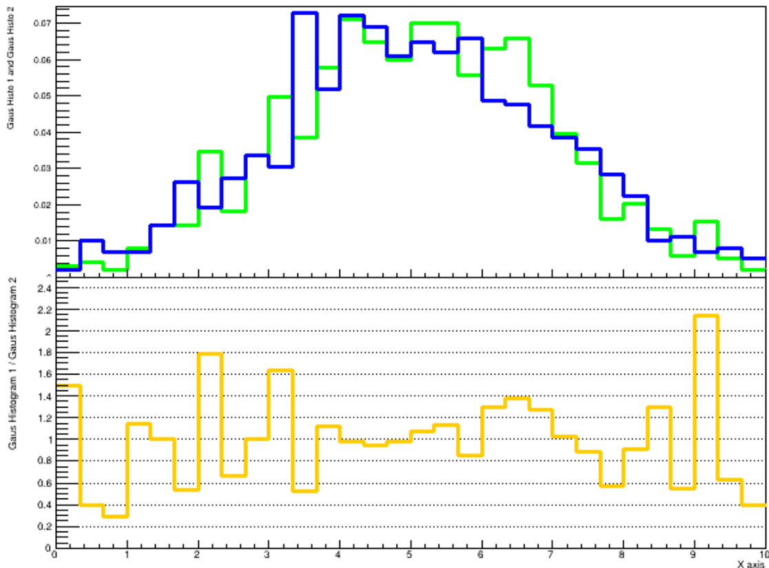
Figure 19: Adding and dividing Histograms
