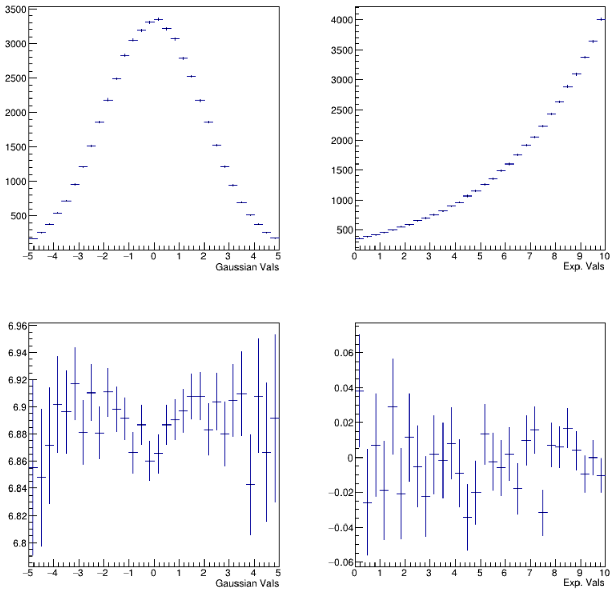
Figure 21: 2D Histograms example2
